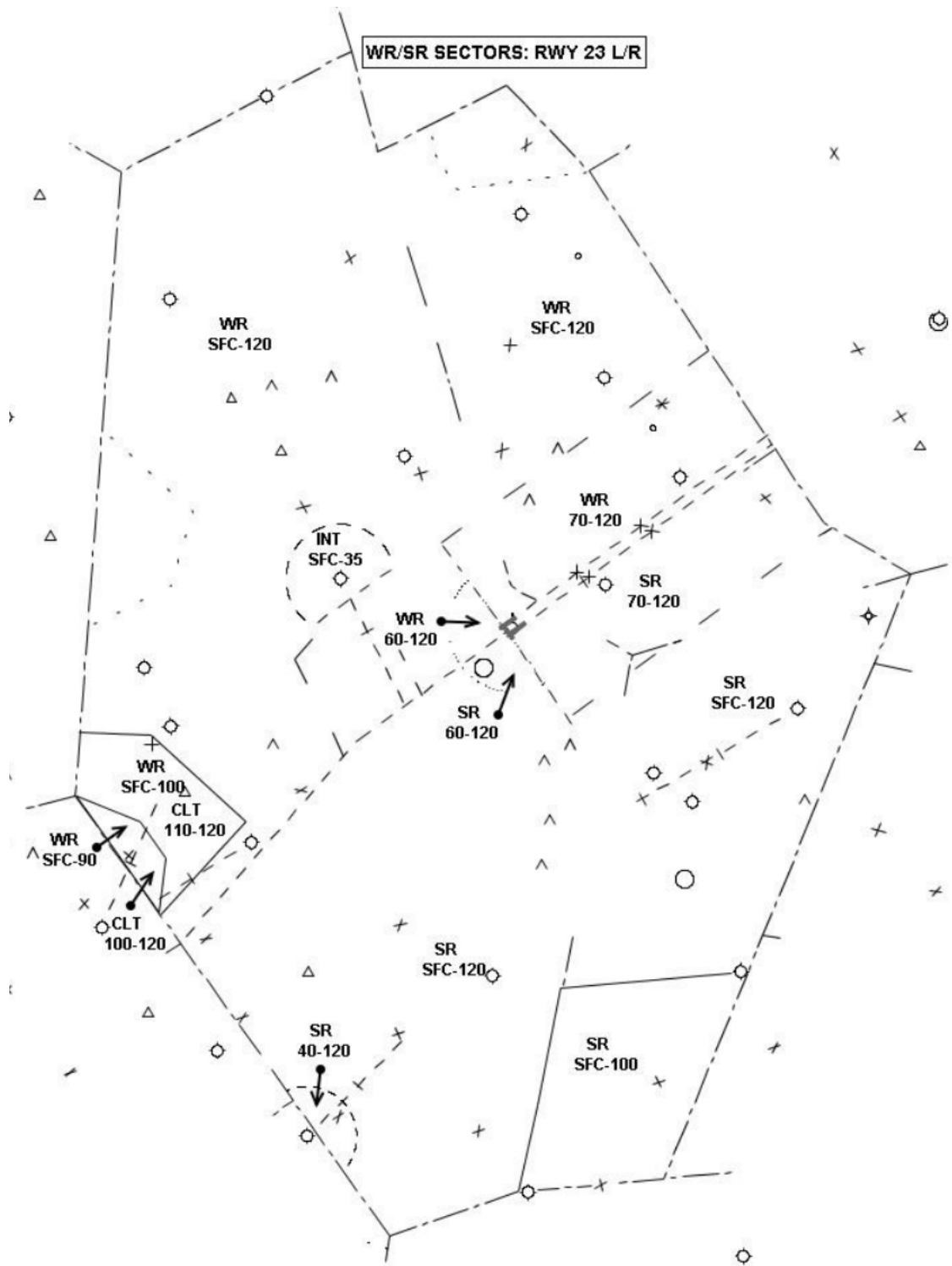
Figure 1-3-1. West/South Radar Airspace (2 Way, Runway 23L/R In Use)
