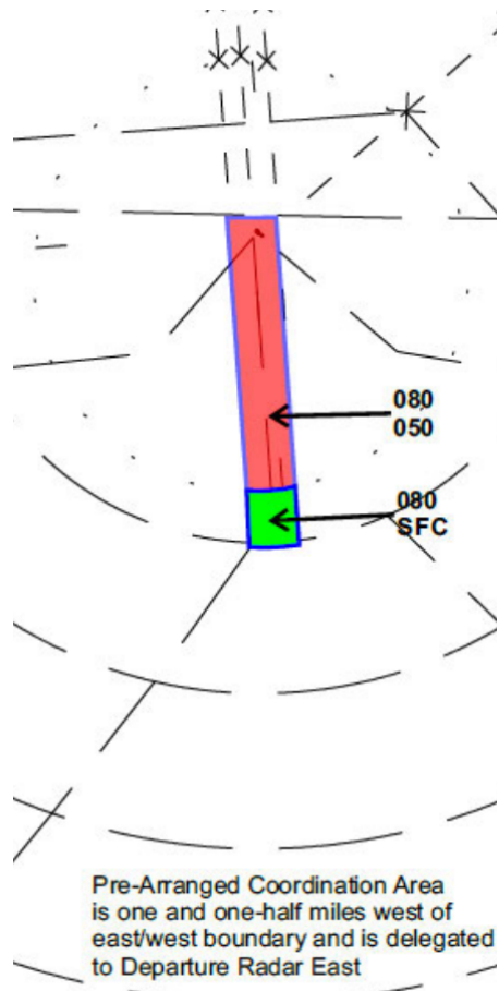
Figure 4-2-5. Departure Radar East/West Pre-Arranged Coordination Area for Runway 19L Departures
